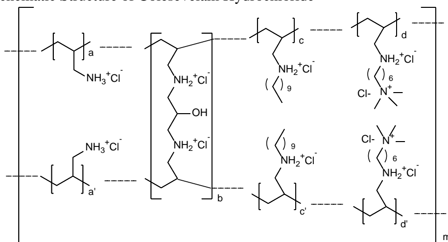
Figure 1. Schematic Structure of Colesevelam Hydrochloride 1
